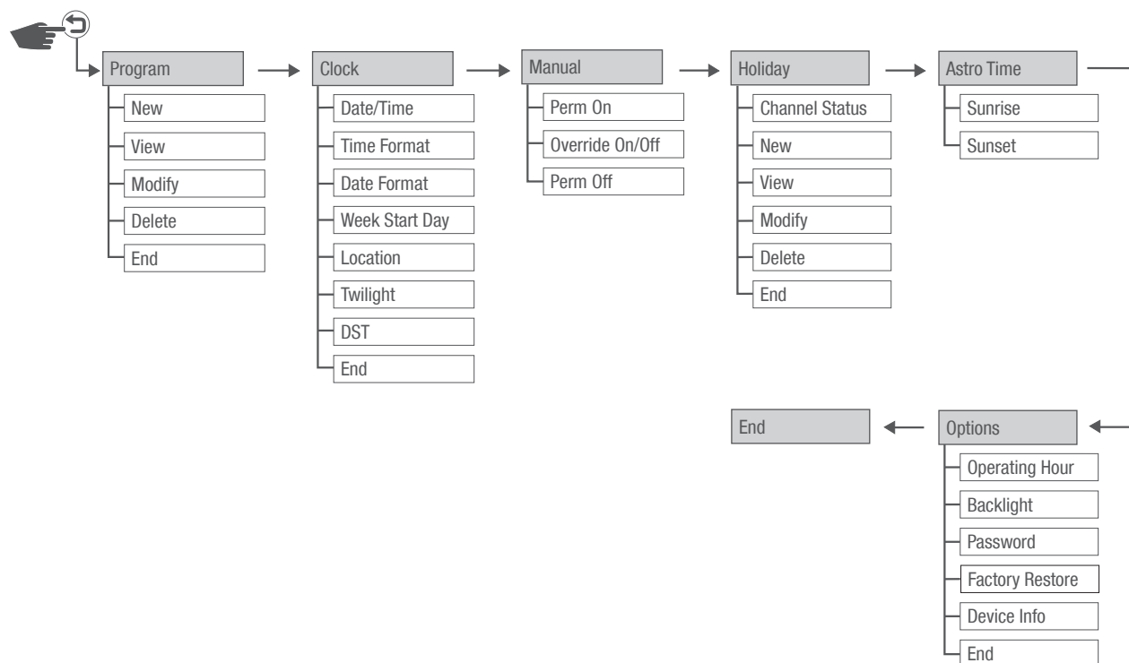
Fig. 3: Menu structure
