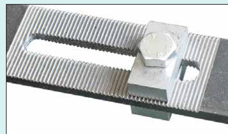
Inbuilt mechanical stops
