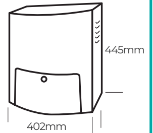
METAL COVER
